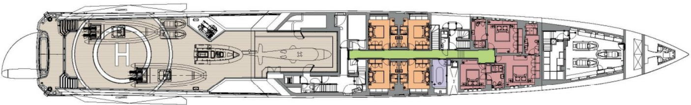
MAIN DECK
