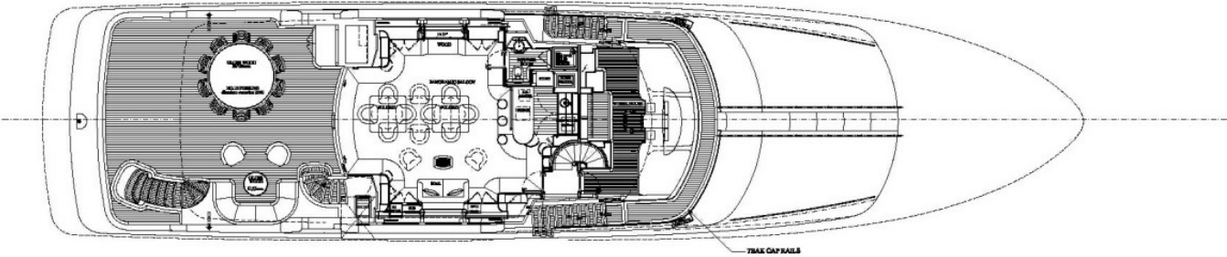
BRIDGE DECK
