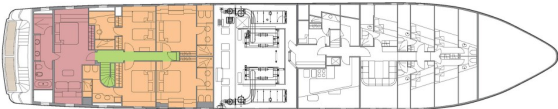
LOWER DECK
