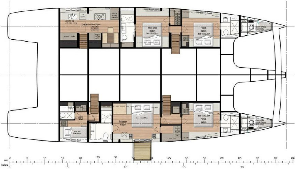
General Arrangement - Lower Deck
