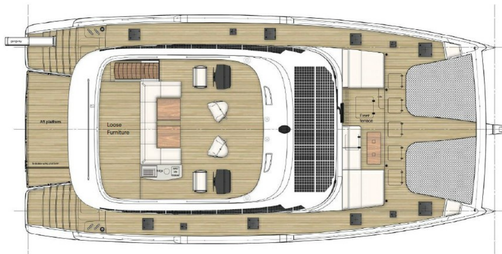
General Arrangement - Fly Bridge
