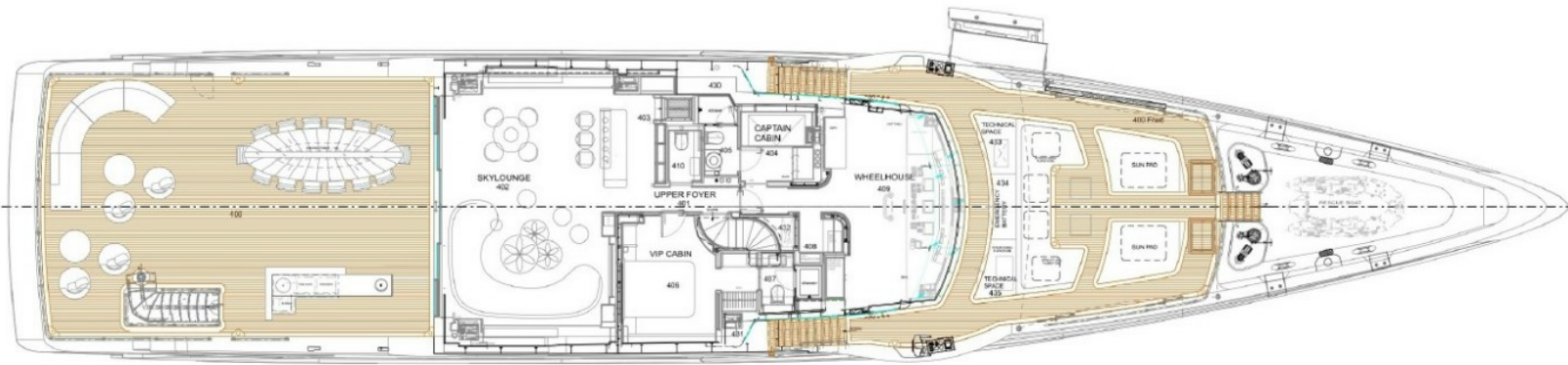
BRIDGE DECK (+700m from B.L.)
