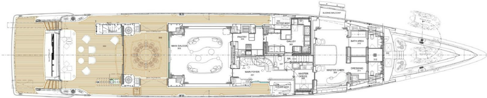
MAIN DECK (+4450m from B.L.)
