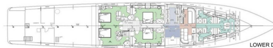
LOWER DECK
