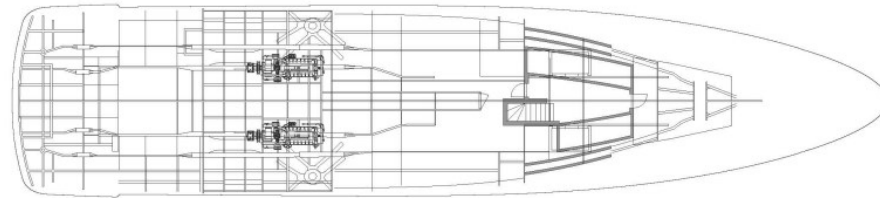
BOTTOM DECK
