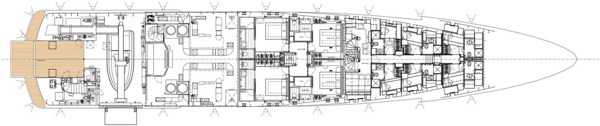
Lower Deck
