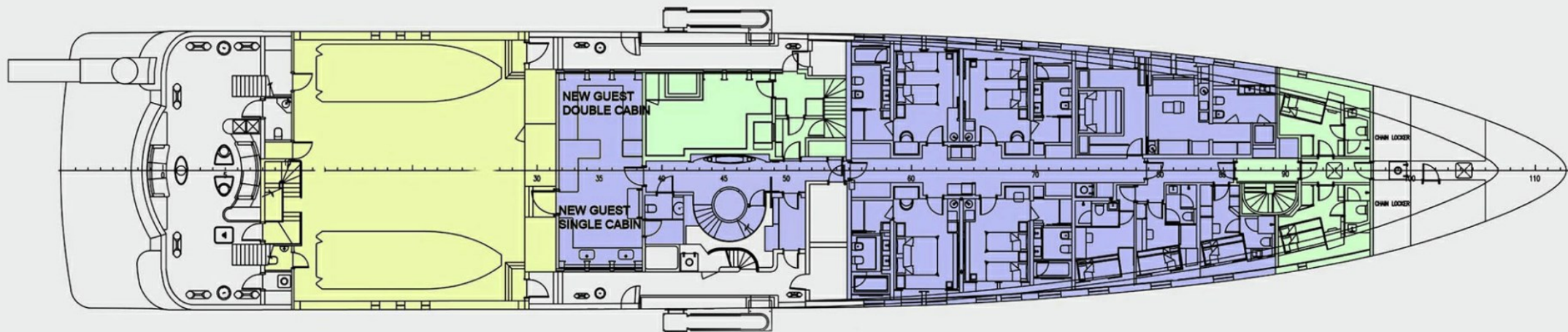
MAIN DECK
