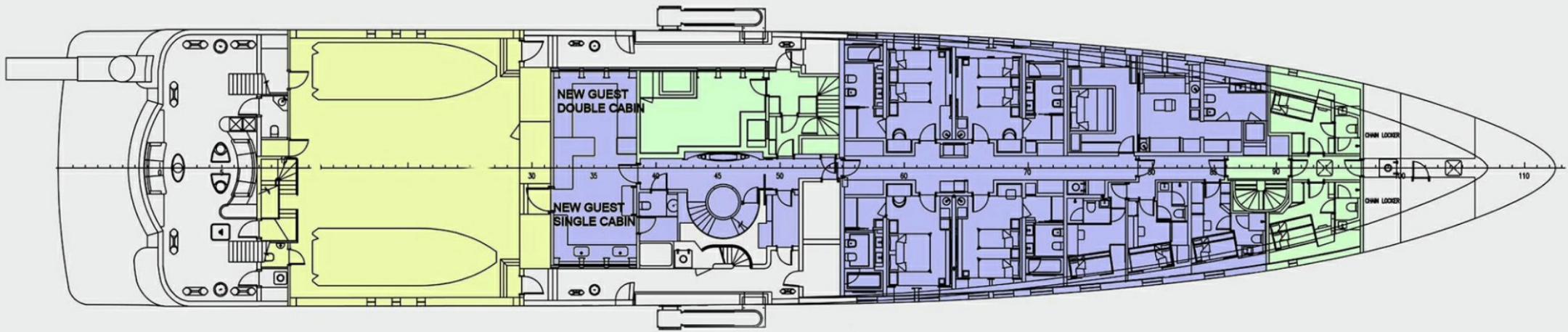
MAIN DECK
