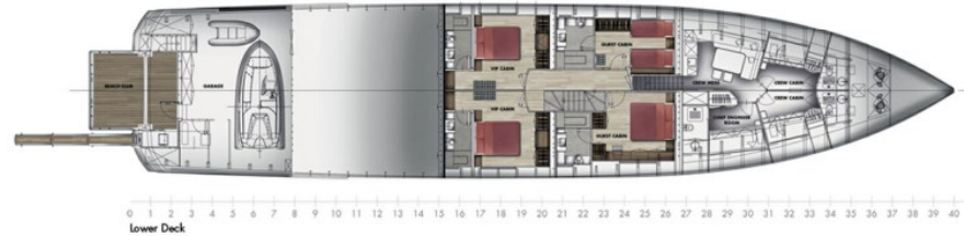
Lower Deck
