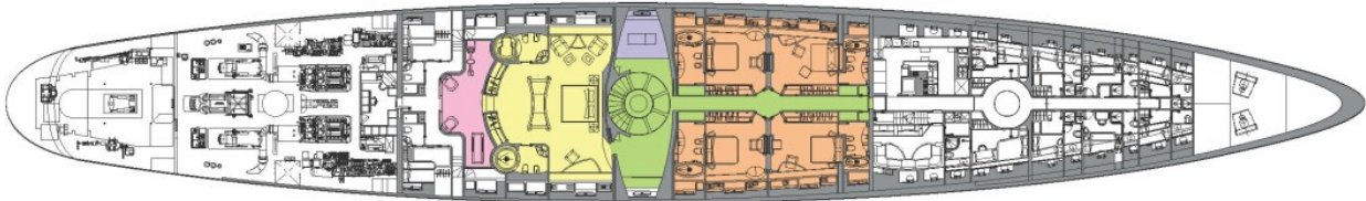
LOWER DECK
