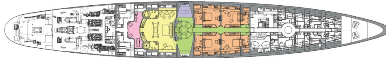
LOWER DECK
