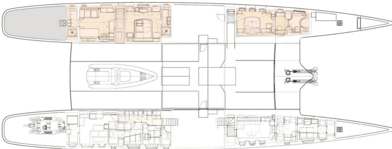
CABIN DECK
