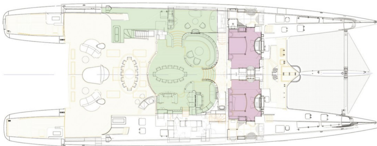
MAIN DECK
