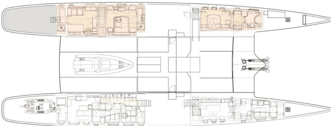
CABIN DECK
