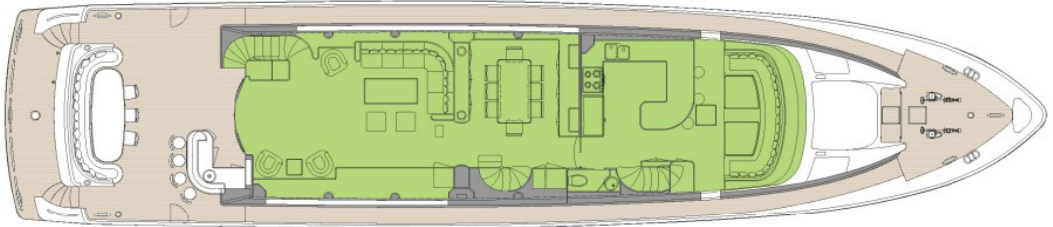
MAIN DECK
