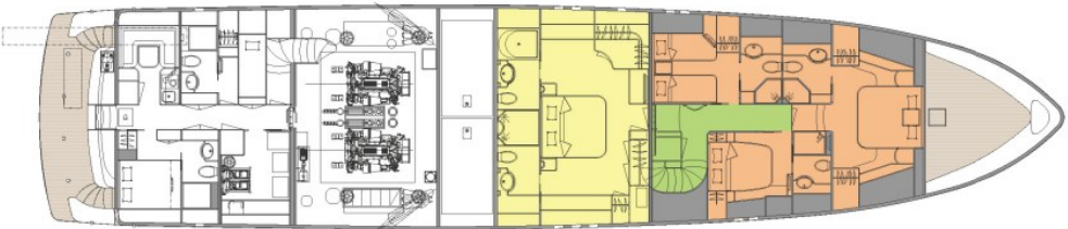
FLOOR DECK
