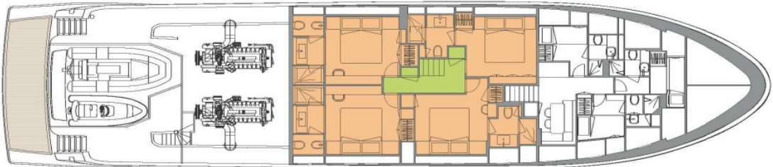
MAIN DECK
