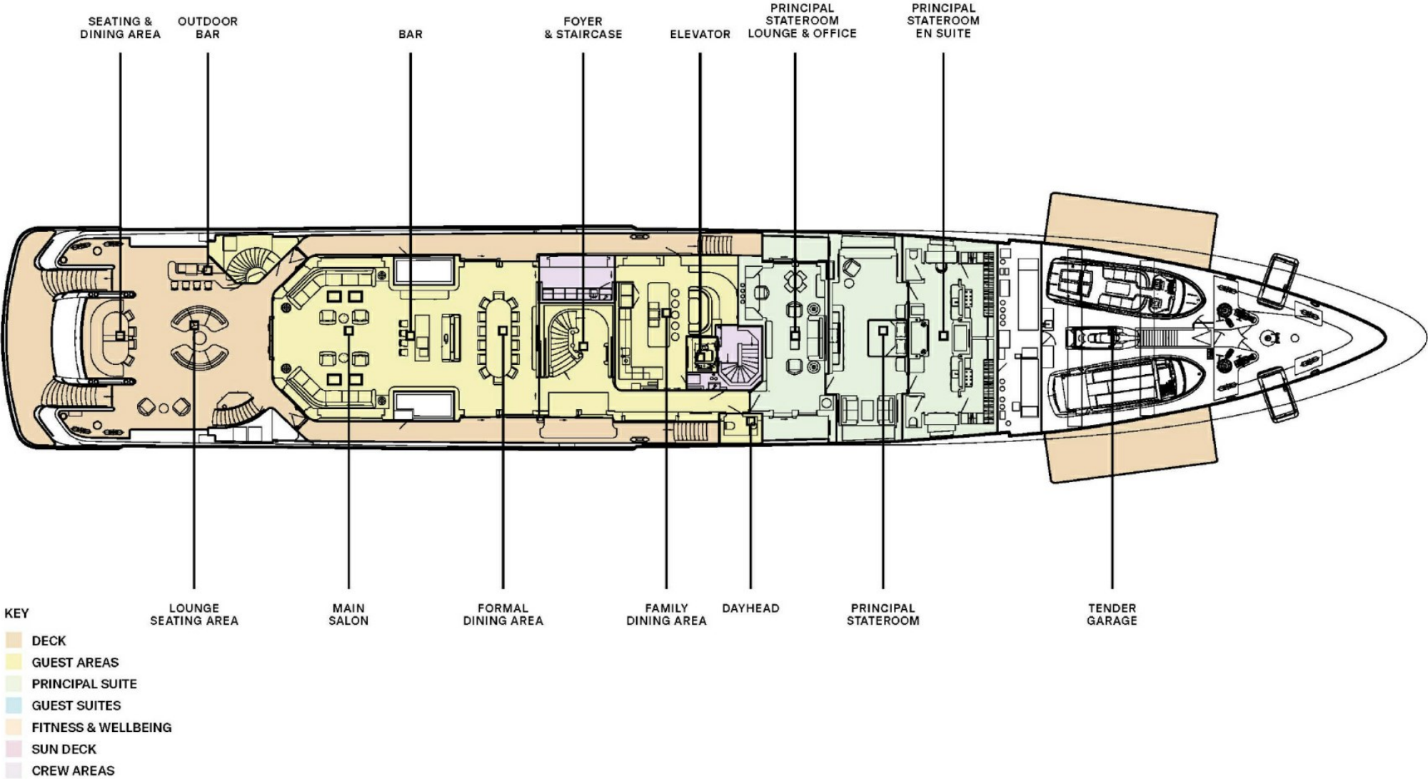
YACHT LAYOUT
