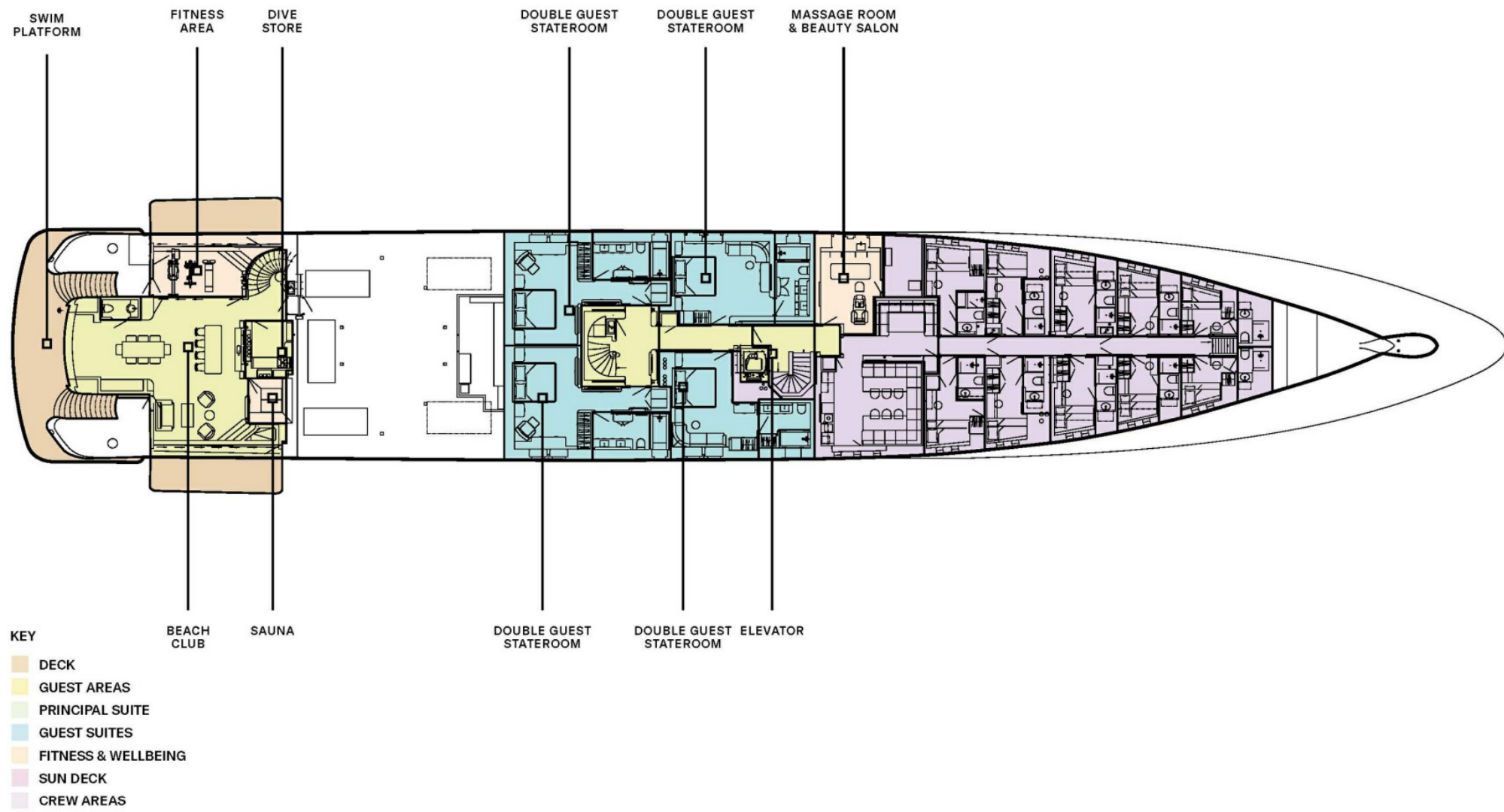
YACHT LAYOUT
