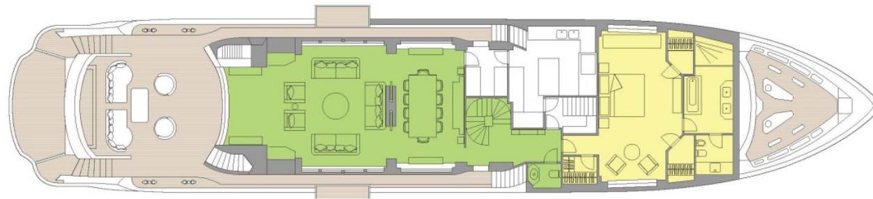
MAIN DECK
