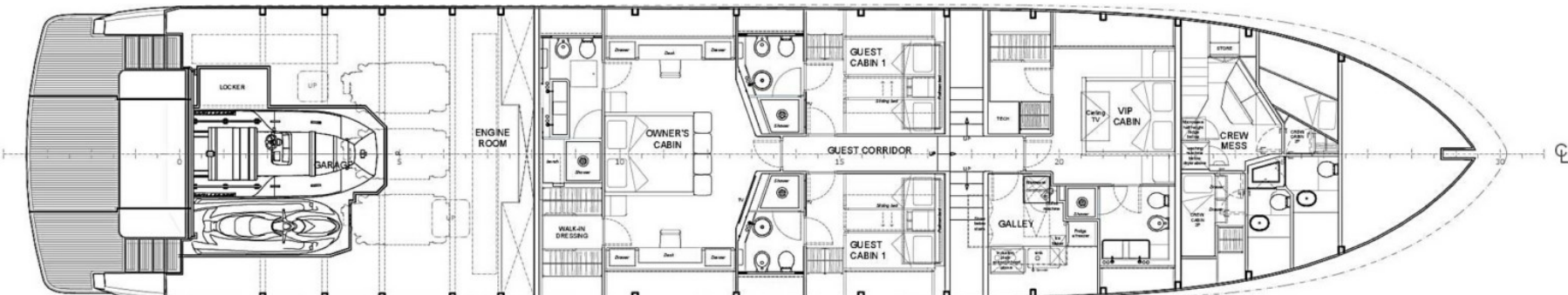
MAIN DECK
